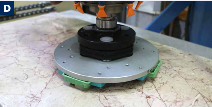
EN Flexible tray Ø330 mm 4 Frankfurt segments FR Plateau souple Ø330 mm 4 segments Frankfurt DE Weiche Platte Ø330 mm 4 Segmente Frankfurt ES Bandeja flexible Ø330 mm 4 segmentos Frankfurt
